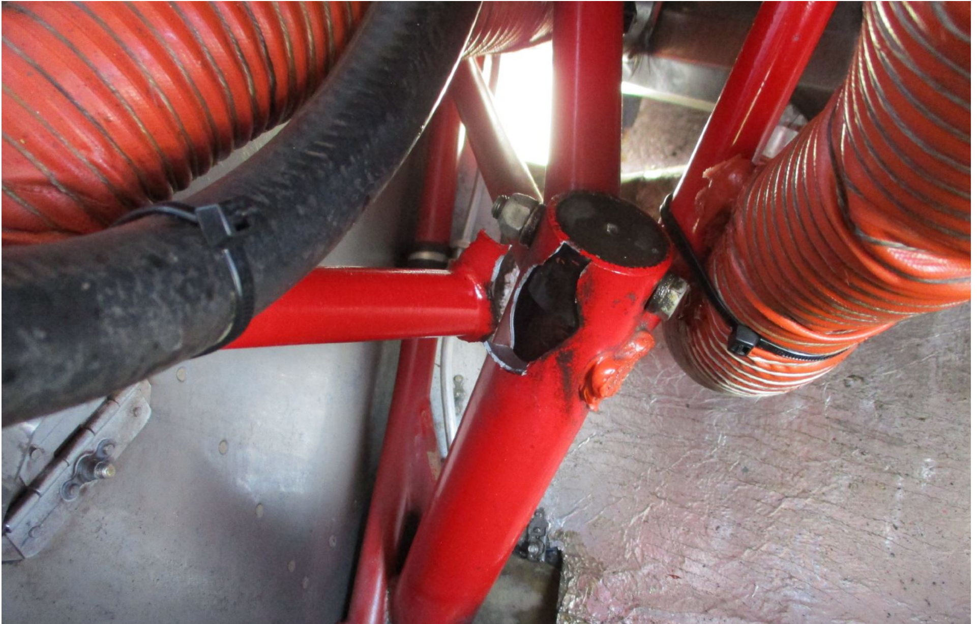
Photo 1 – View of damaged engine mount (courtesy of the FAA)
