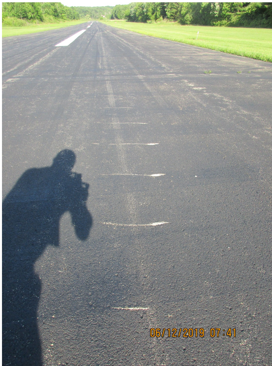
Photo 1 – View of propeller scars on the runway (Photo courtesy of the FAA)
