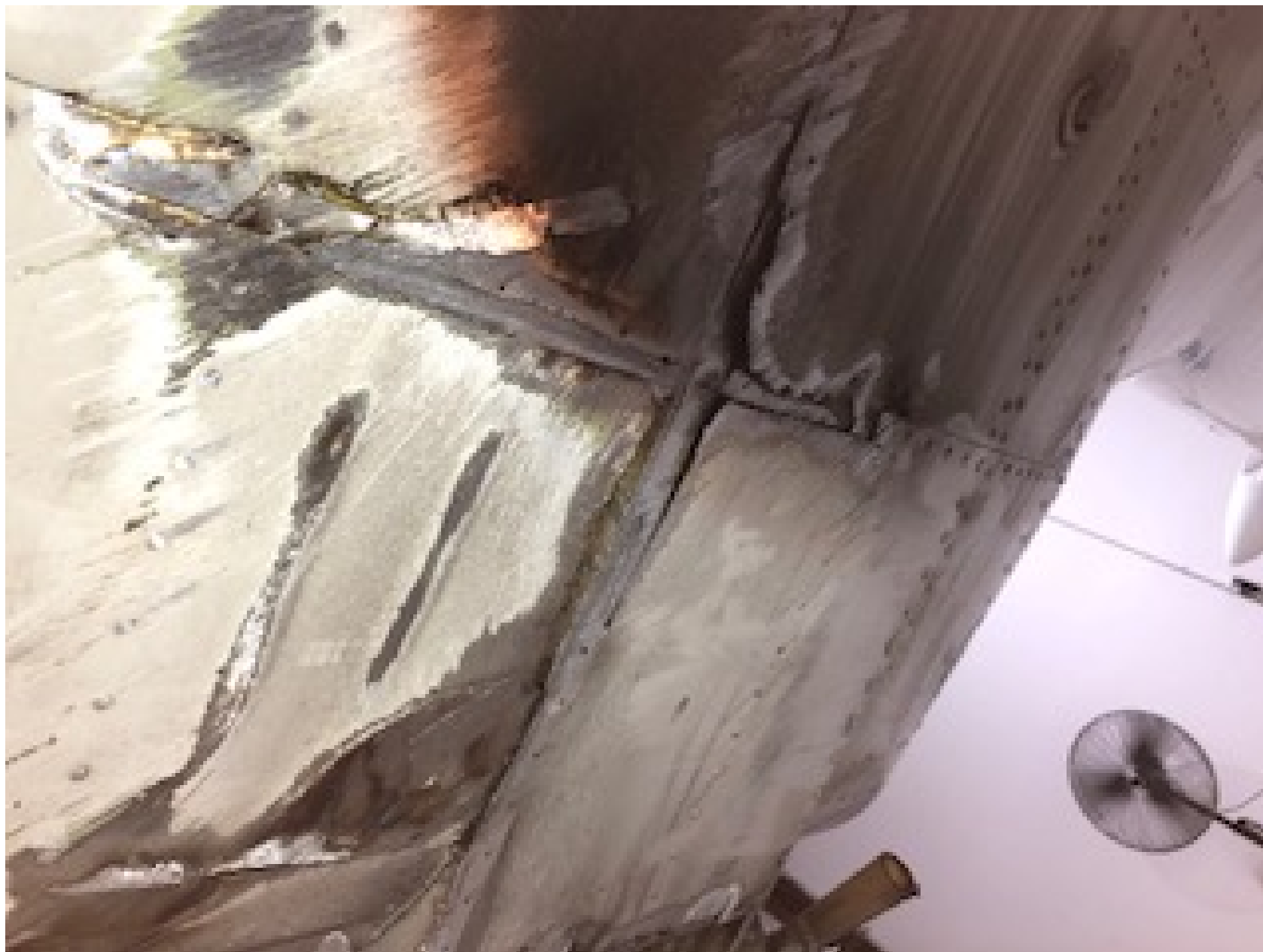
Photo 1 – View of the damage to the lower fuselage (Courtesy of FAA)
