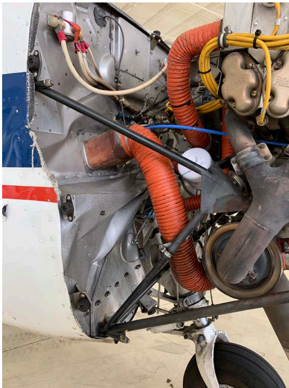
Photo 1 – View of damaged firewall and engine mount frame (courtesy of the airframe and powerplant mechanic)
