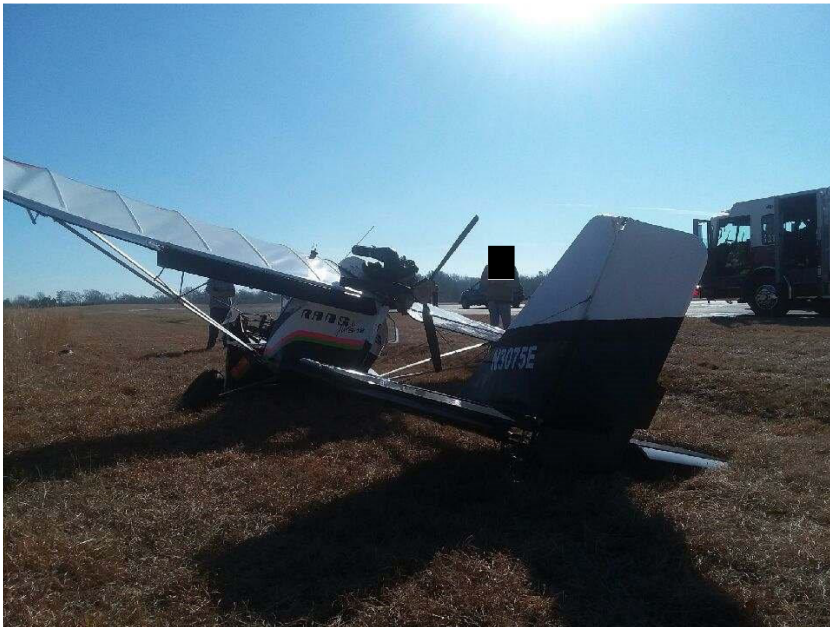
Photo 5 - View of empennage damage (photo courtesy of the FAA).
