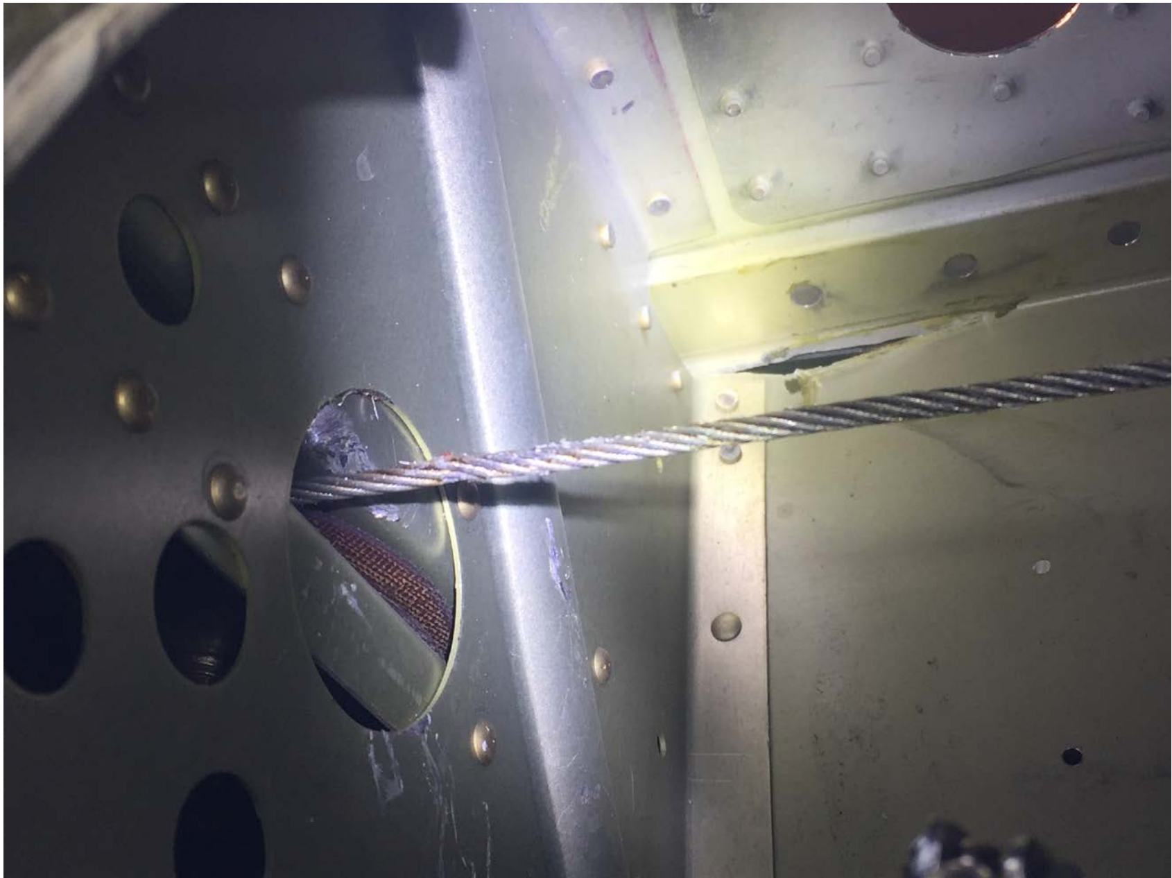
Photo 1 – View of damaged right-wing aft spar (courtesy of the FAA)
