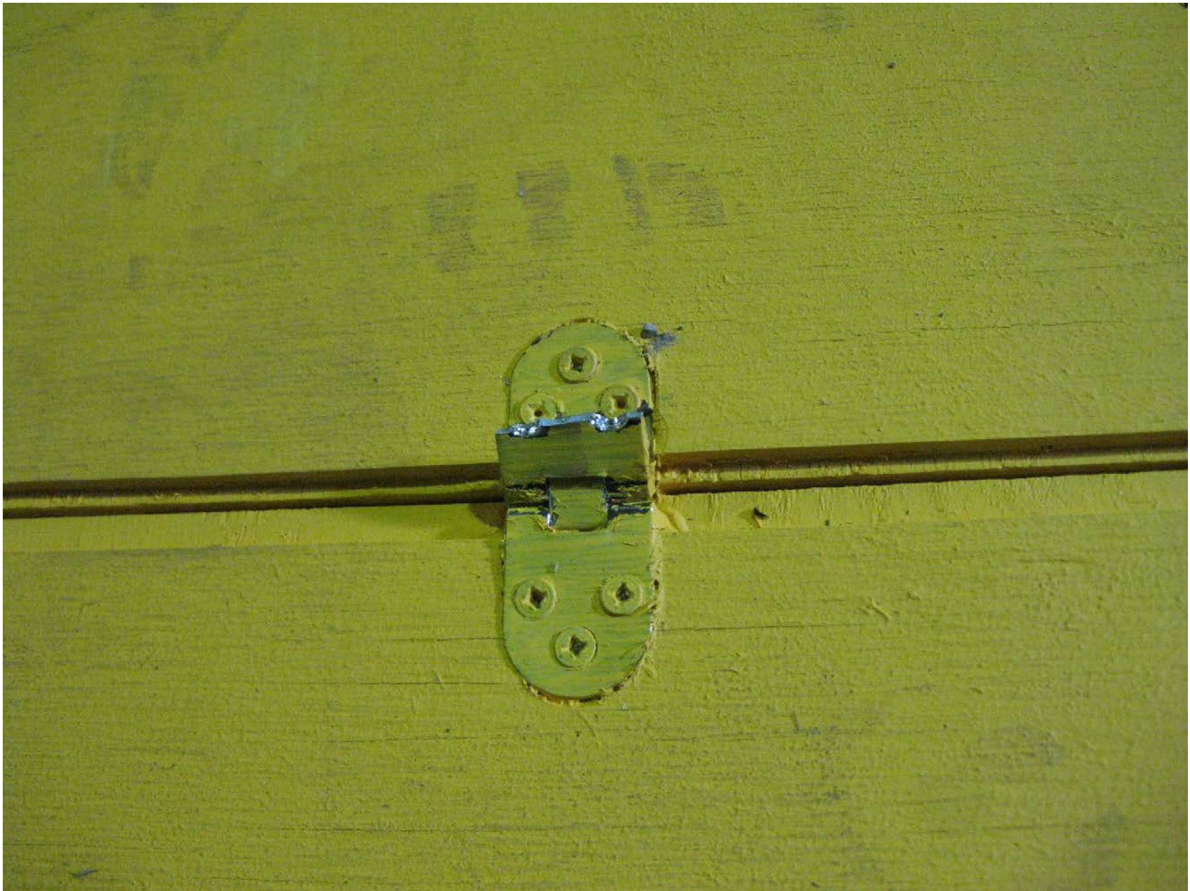
Photo 2 – View of failed hinge on owner-made dolly (Photo courtesy of the FAA)
