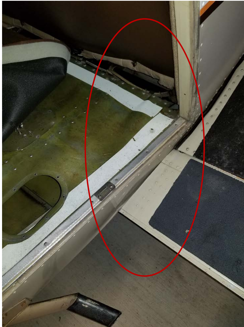
Photo 2 – View of damaged baggage compartment floorboard (Photo courtesy of the FAA)
