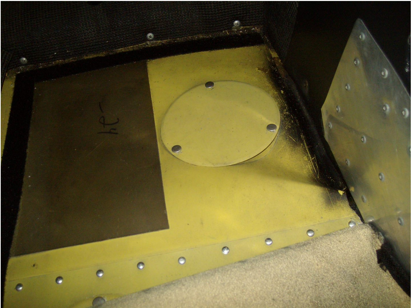
Photo 1 – View of damaged floorboards (Photo courtesy of the flight school)
