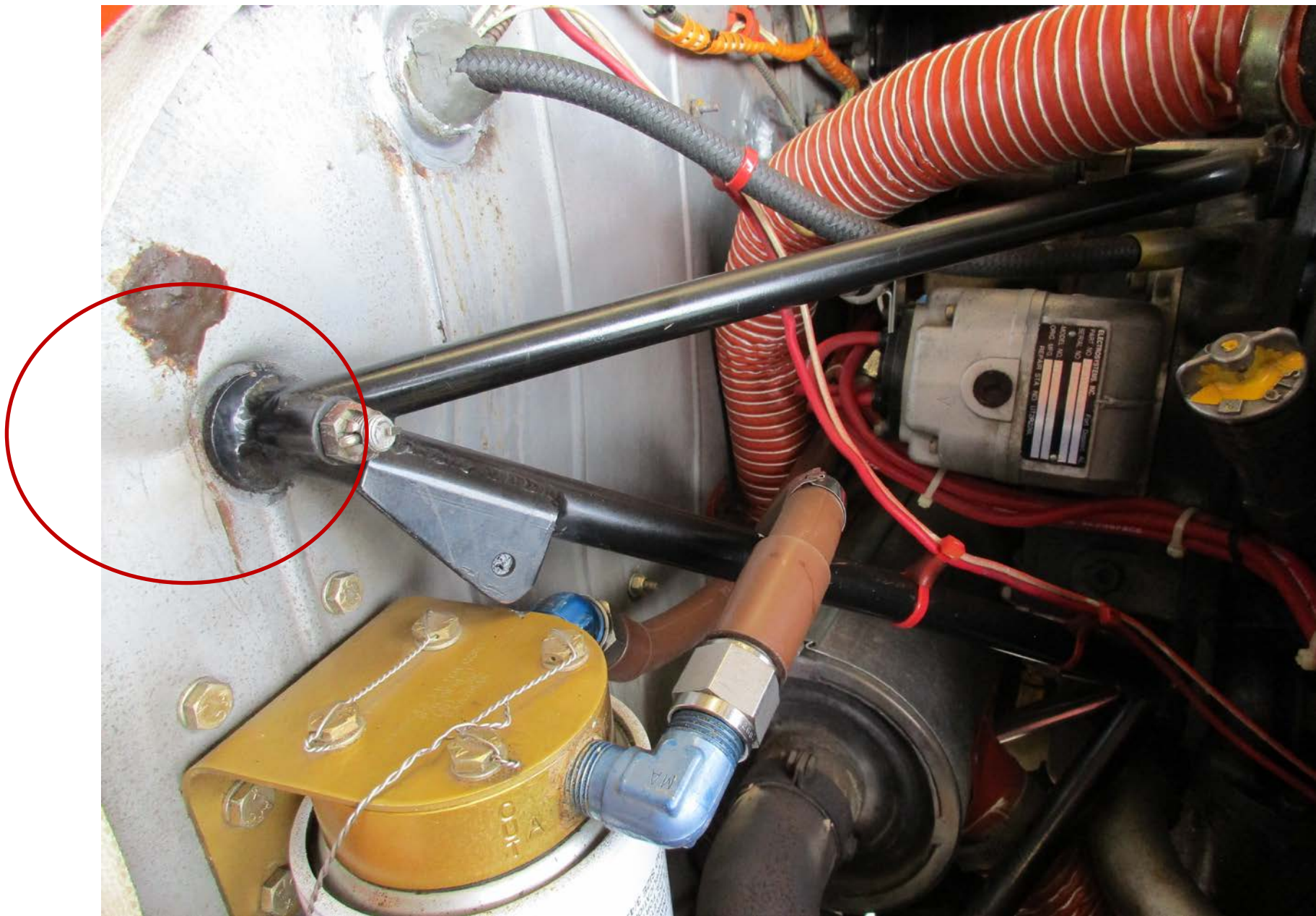
Photo 2 – View of wrinkle damage to firewall (courtesy of the FAA)
