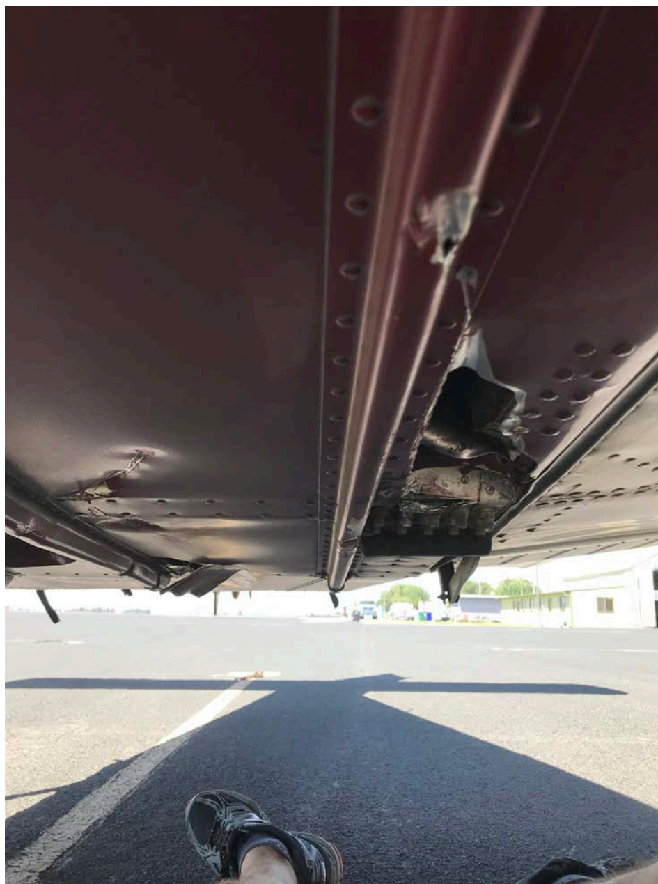
Photo 1 – View of damage to the lower fuselage (Courtesy of FAA)
