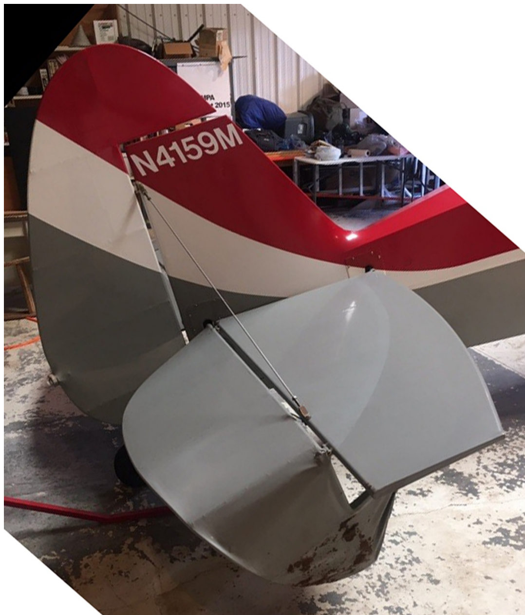
Photo 2 – View of damaged right elevator (Photo courtesy of the pilot’s attorney)
