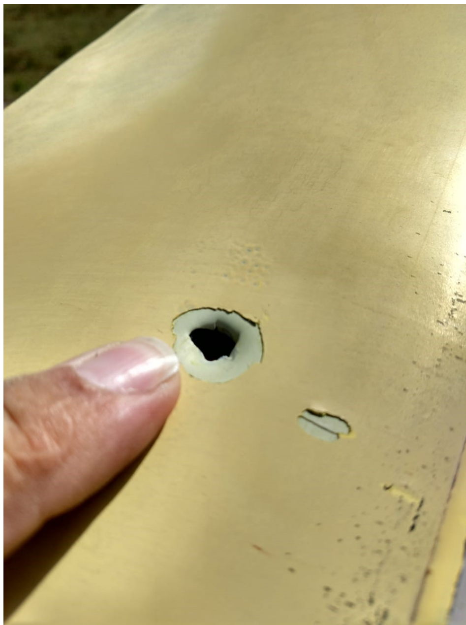
Photo 2 – View of a hole in the top of the main rotor blade (Courtesy of FAA)
