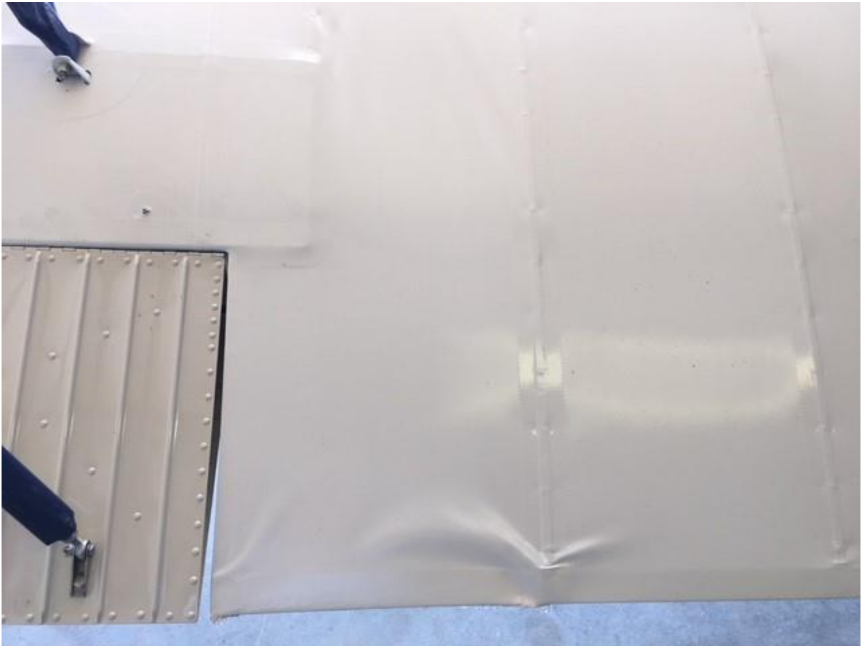
Photo 2 – Top view of damaged lower left wing (Photo courtesy of the FAA)
