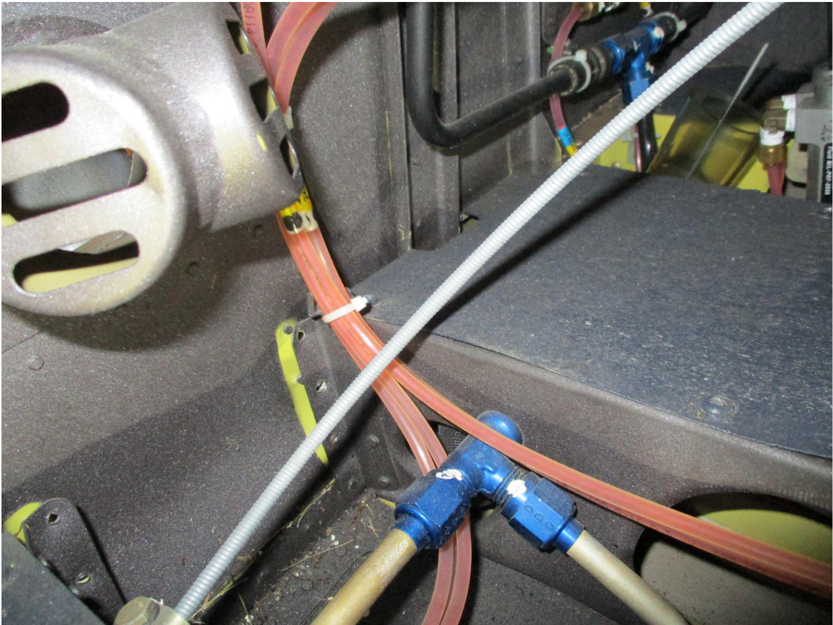
Photo 2 – View of buckled interior floorboard (Photo courtesy of the FAA)
