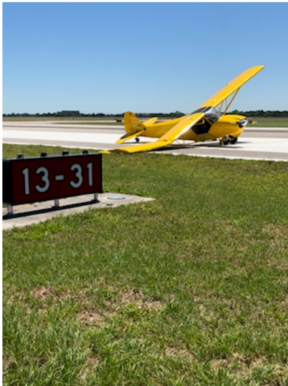
Photo 1 – View of damaged right wing (Photo courtesy of the FAA)
