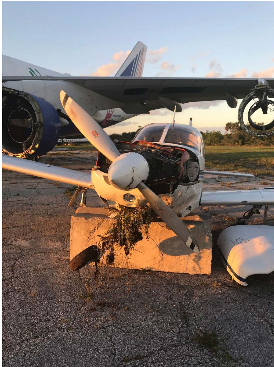
Photo 1 – View of damage to the nose section (Courtesy of FAA)
