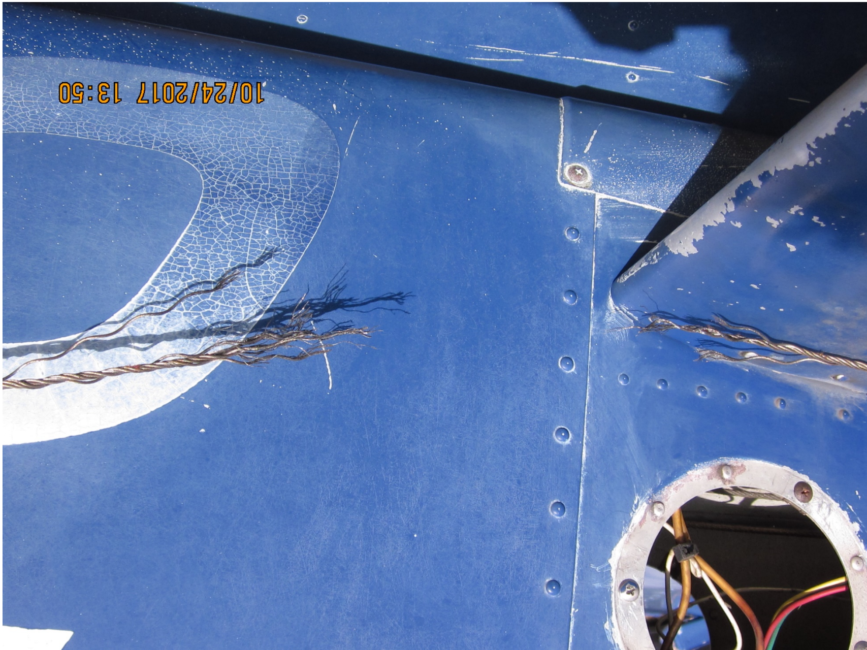
Photo 2 – View of separated rudder cable (photo courtesy of the FAA)
