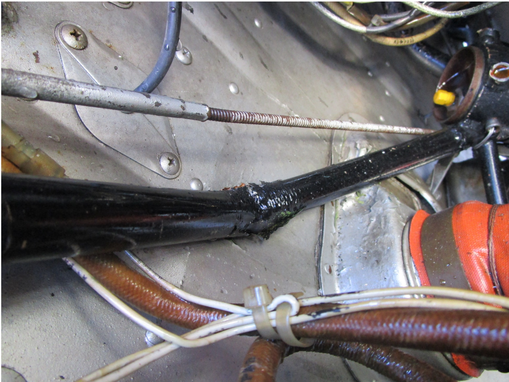
Photo 1 – View of damaged engine mount (photo courtesy of the FAA)
