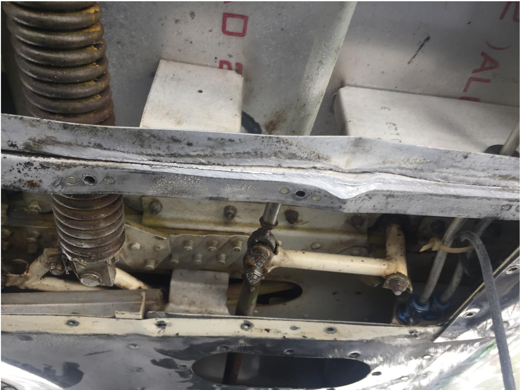
Photo 1 – View of fuselage damage (photo courtesy of the FAA)
