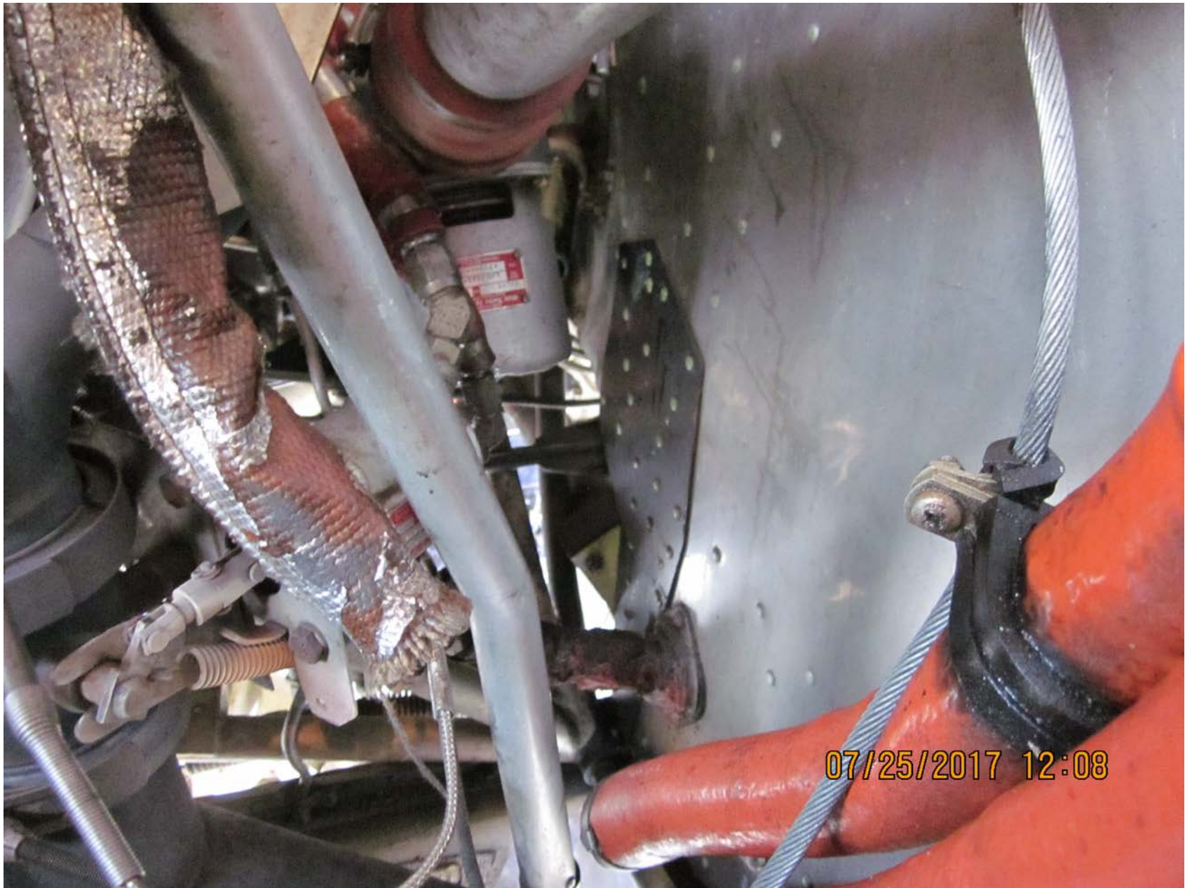
Photo 1 – Substantially Damaged Engine Mount and Firewall (Photo Courtesy of FAA)
