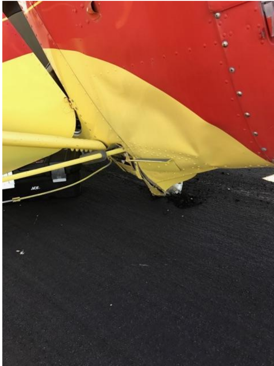
Photo 1 – Front view of right landing gear and fuselage (Photo courtesy of the FAA)
