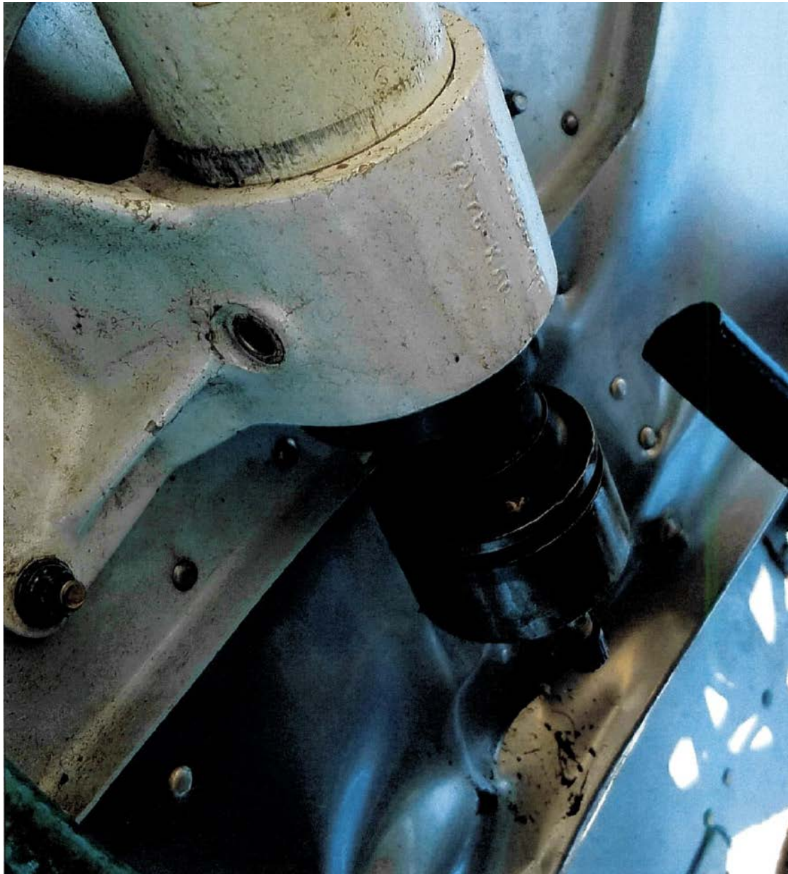
Photo 1 – View of damage to the firewall (Courtesy of the Operator)
