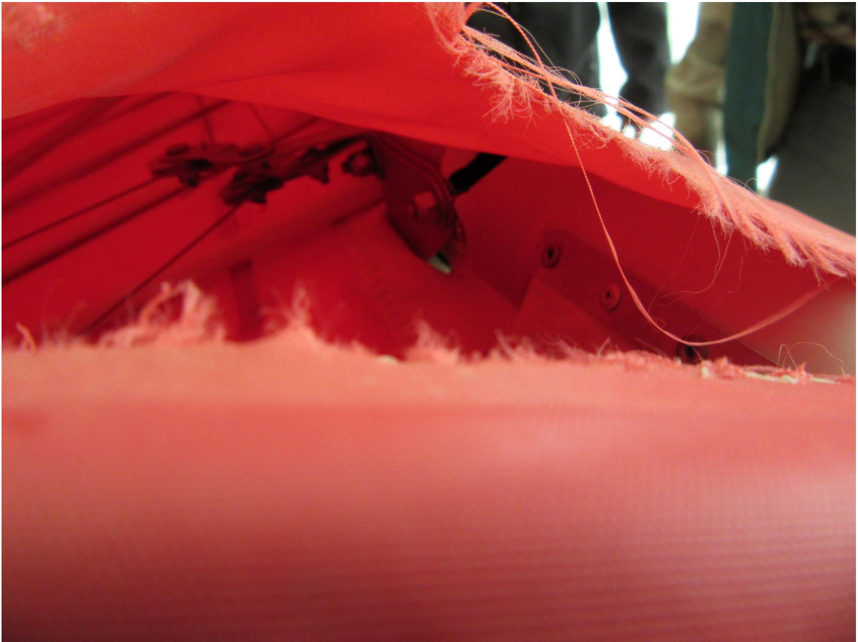
Photo 1 – View of right wing damage (photo courtesy of the FAA)
