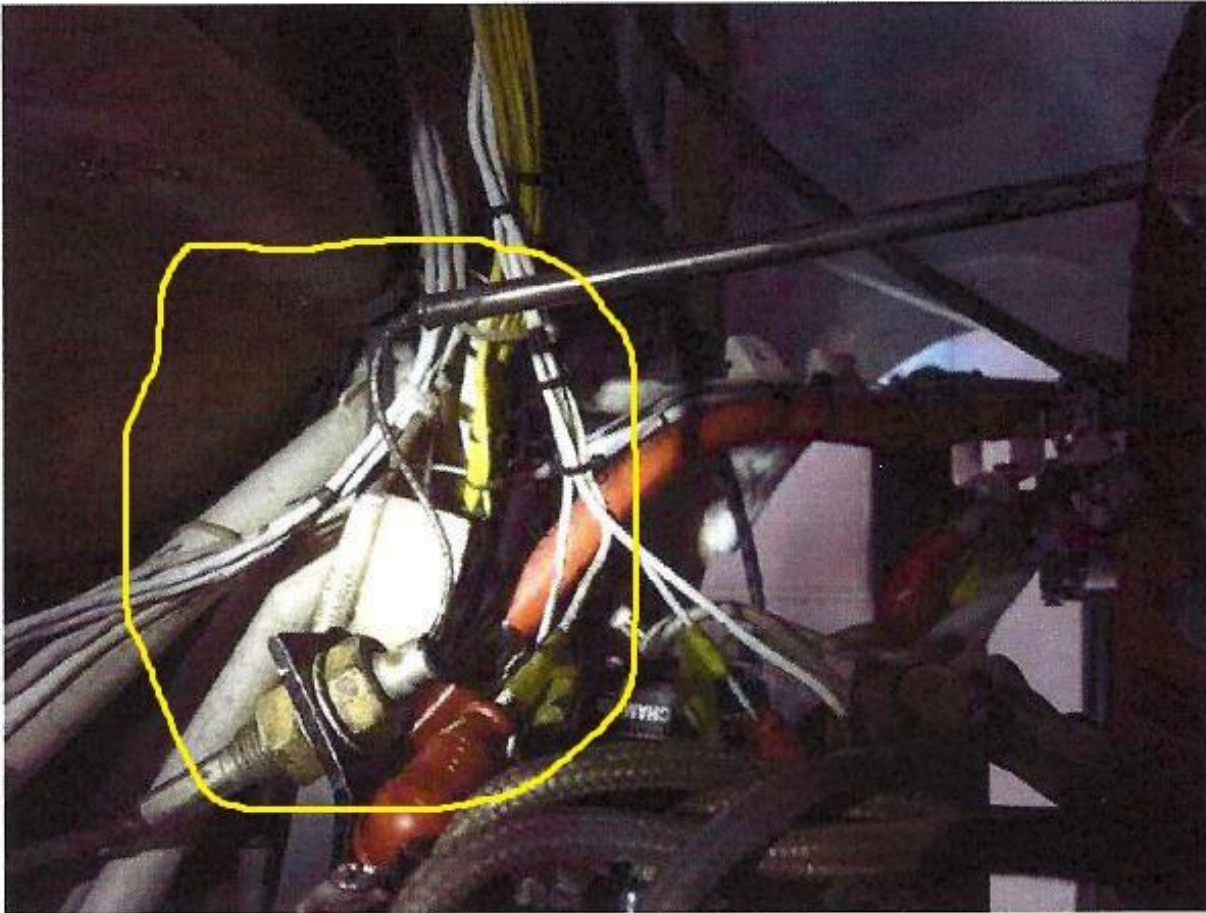
Throttle cable at idle
