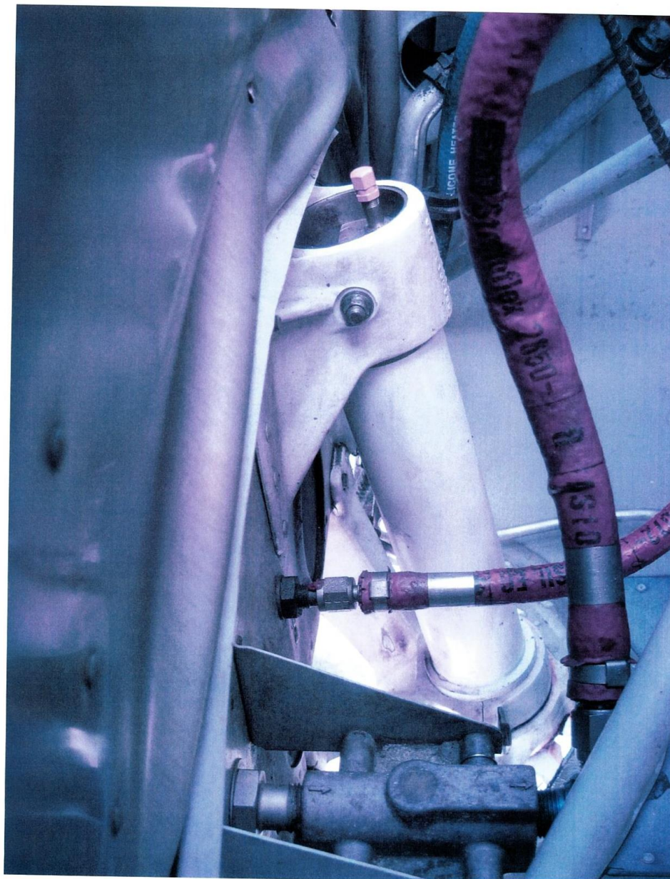
Photo 1 – View of damaged firewall (Photo courtesy of the FAA)
