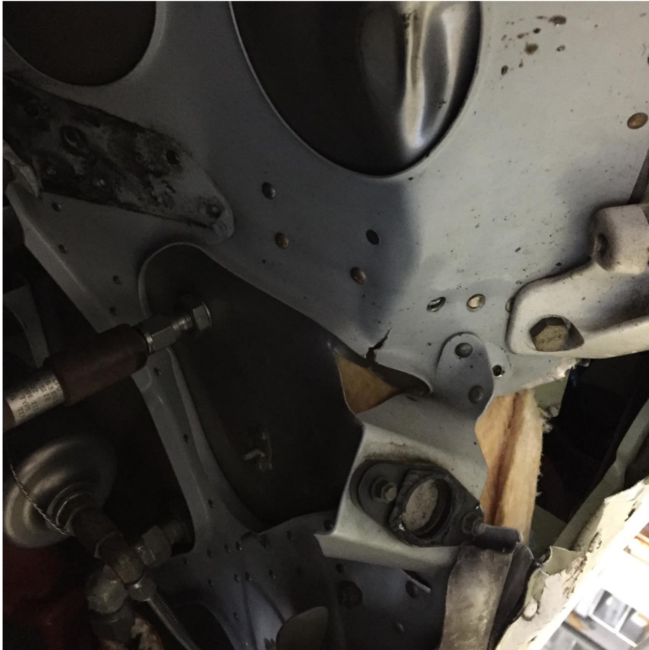
Photo 2 – View of damaged firewall (Photo courtesy of the FAA)
