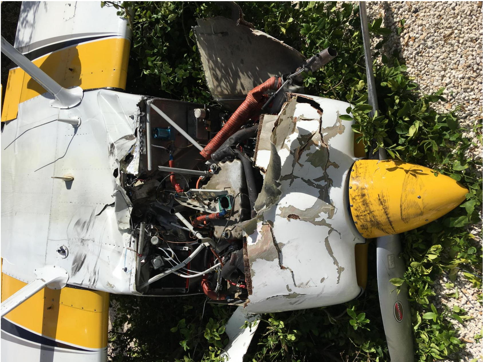
Photo 2 – View of fuselage, firewall, and engine mounts (courtesy of the FAA)
