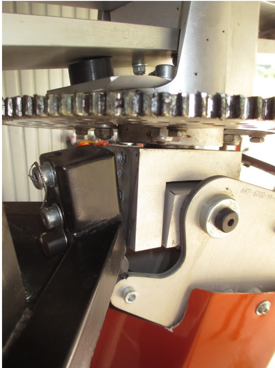
Photo 3 – View of damage to main rotor hub (Courtesy of FAA)
