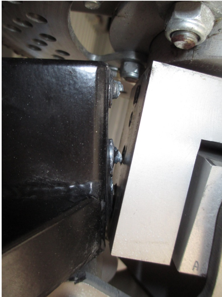
Photo 2 – View of damage to main rotor hub (Courtesy of FAA)
