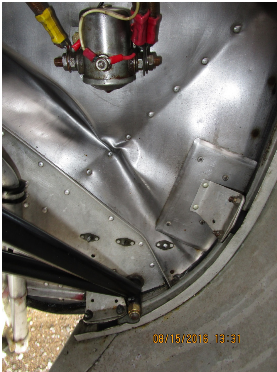
Photo 2 - View of firewall damage (photo courtesy of the FAA)
