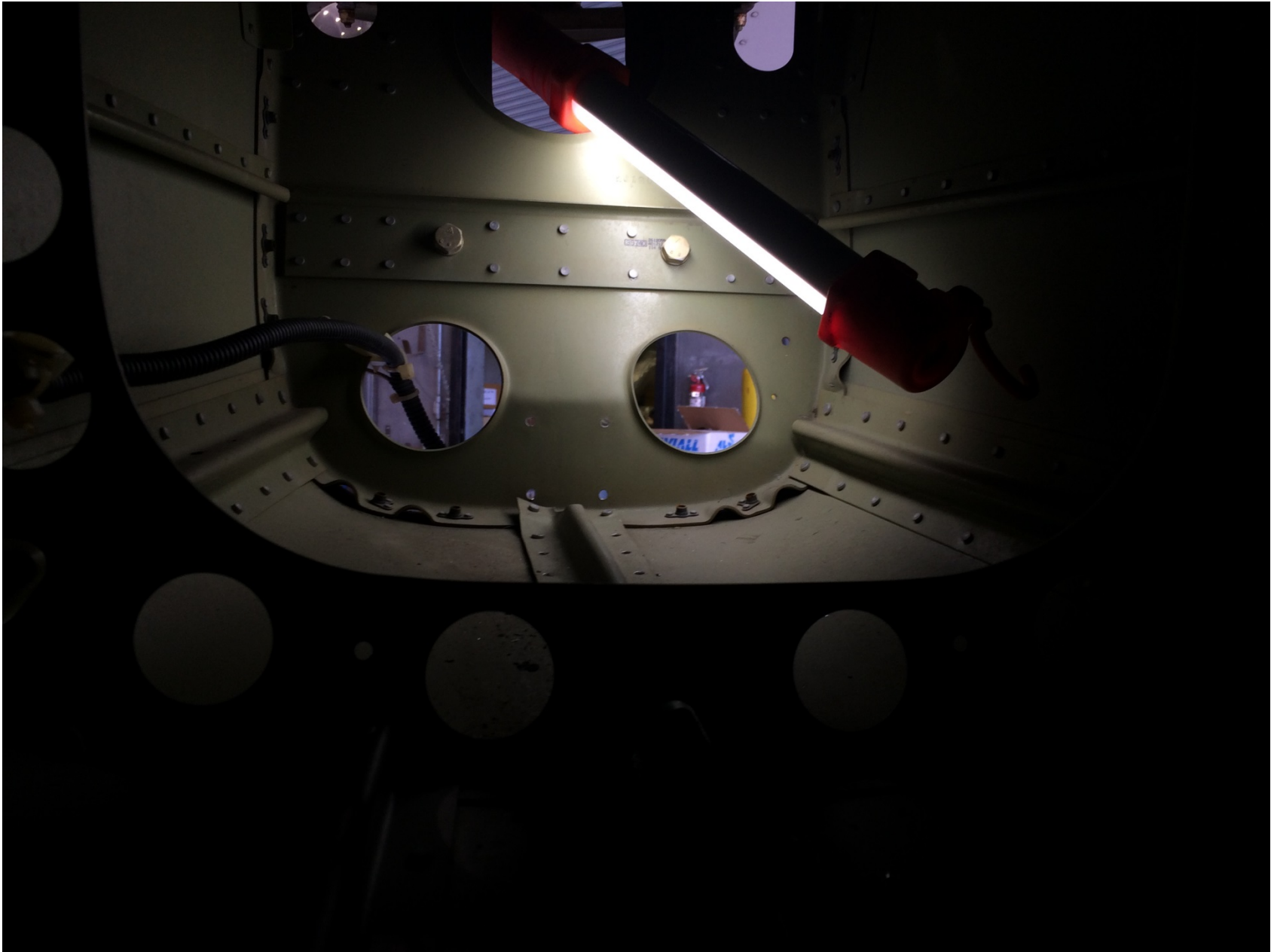
Photo 1 – Substantially Damaged Aft Bulkhead (Photo Courtesy of FAA)
