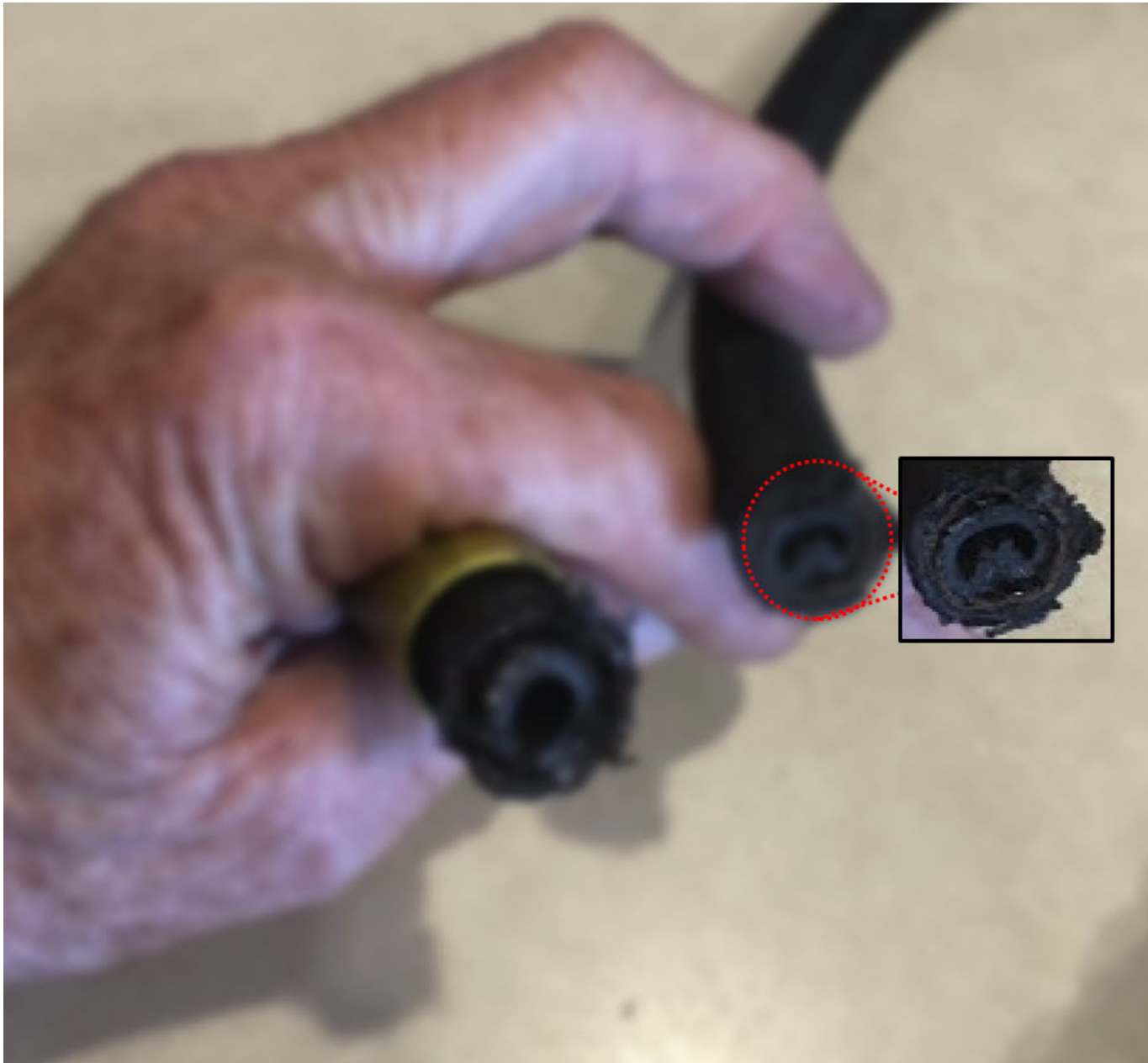
Photo 2 - View of damaged fuel line (photo courtesy of the FAA)
