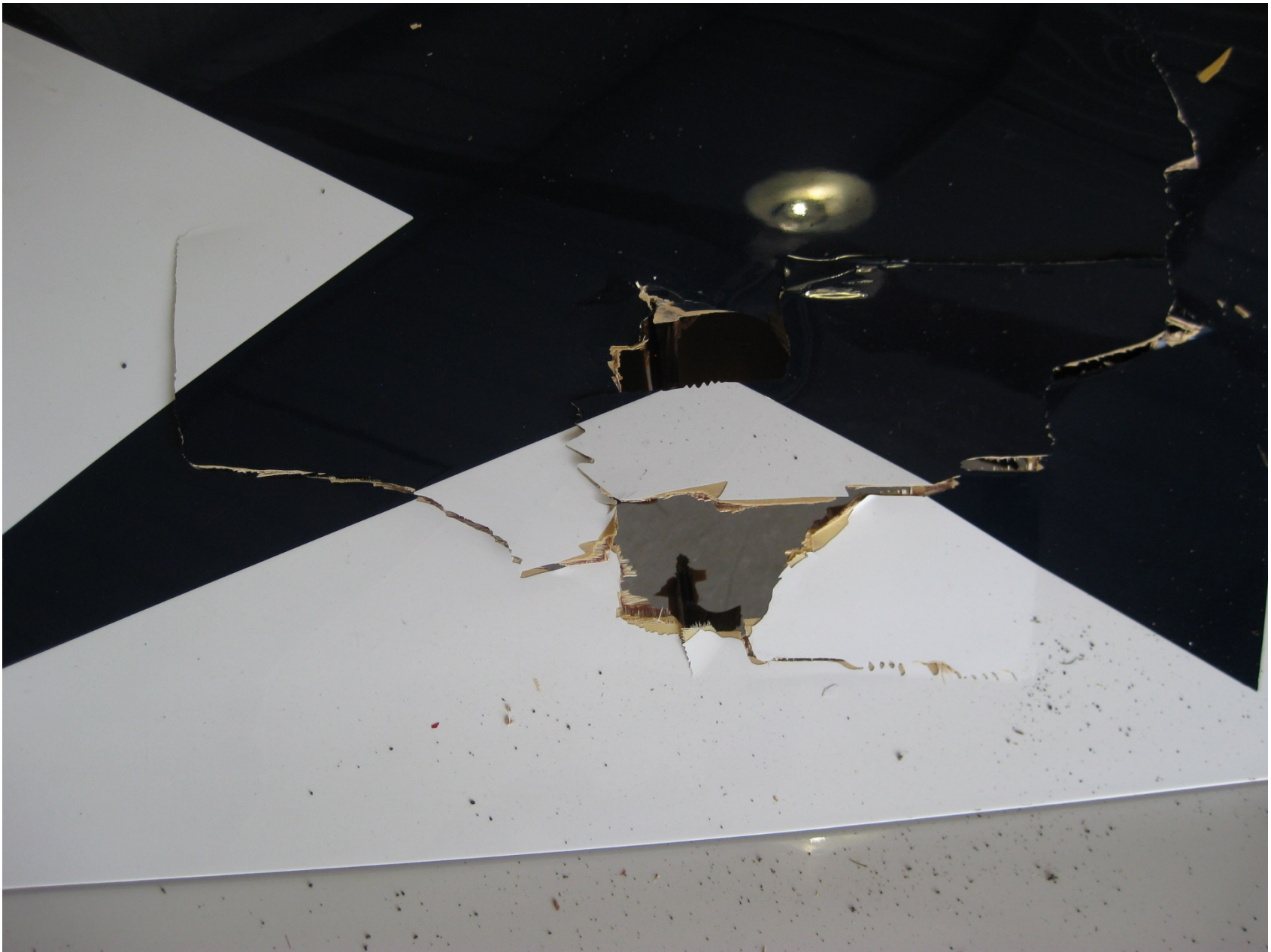
Photo 1 – Left Horizontal Stabilizer (Photo Courtesy of FAA)
