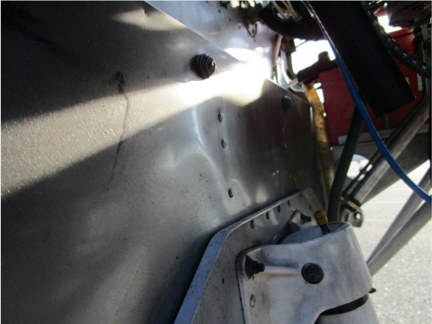
Photo 1 – Substantially Damaged Firewall (Courtesy of FAA)
