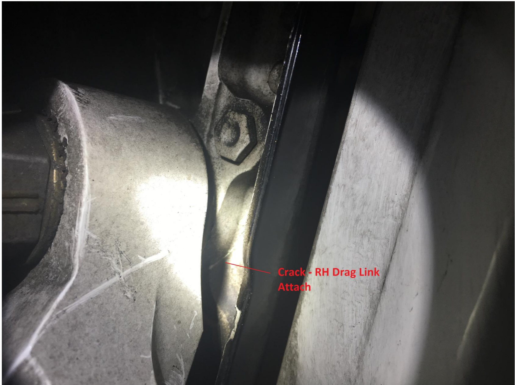
Photo 1 – View of drag link attachment (courtesy of the manufacturer)
