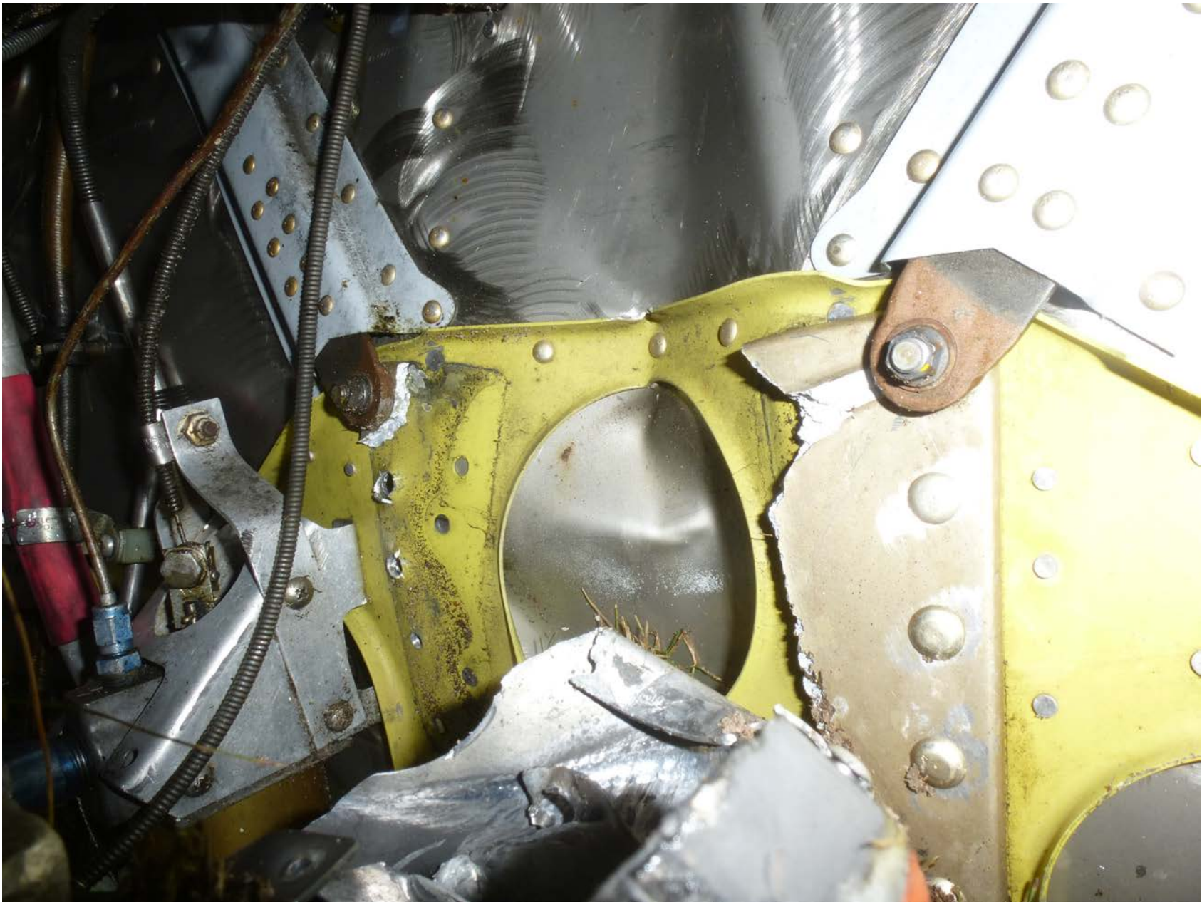
Photo 3 - View of substantial damage to the firewall (photo courtesy of the FAA)
