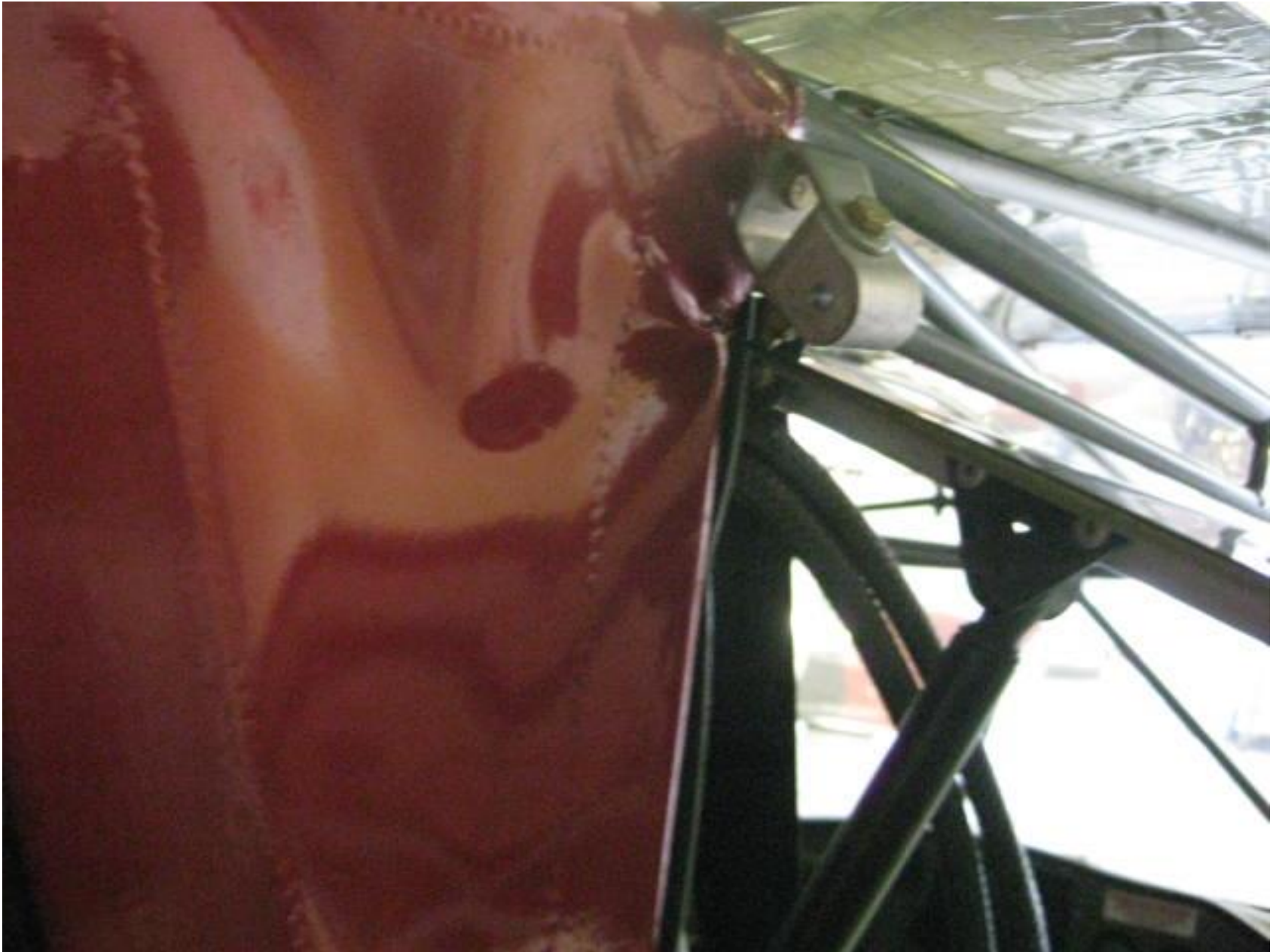
Photo 2 – Close up of damage to the truss structure at the right rear wing root attachment point (Courtesy of FAA)
