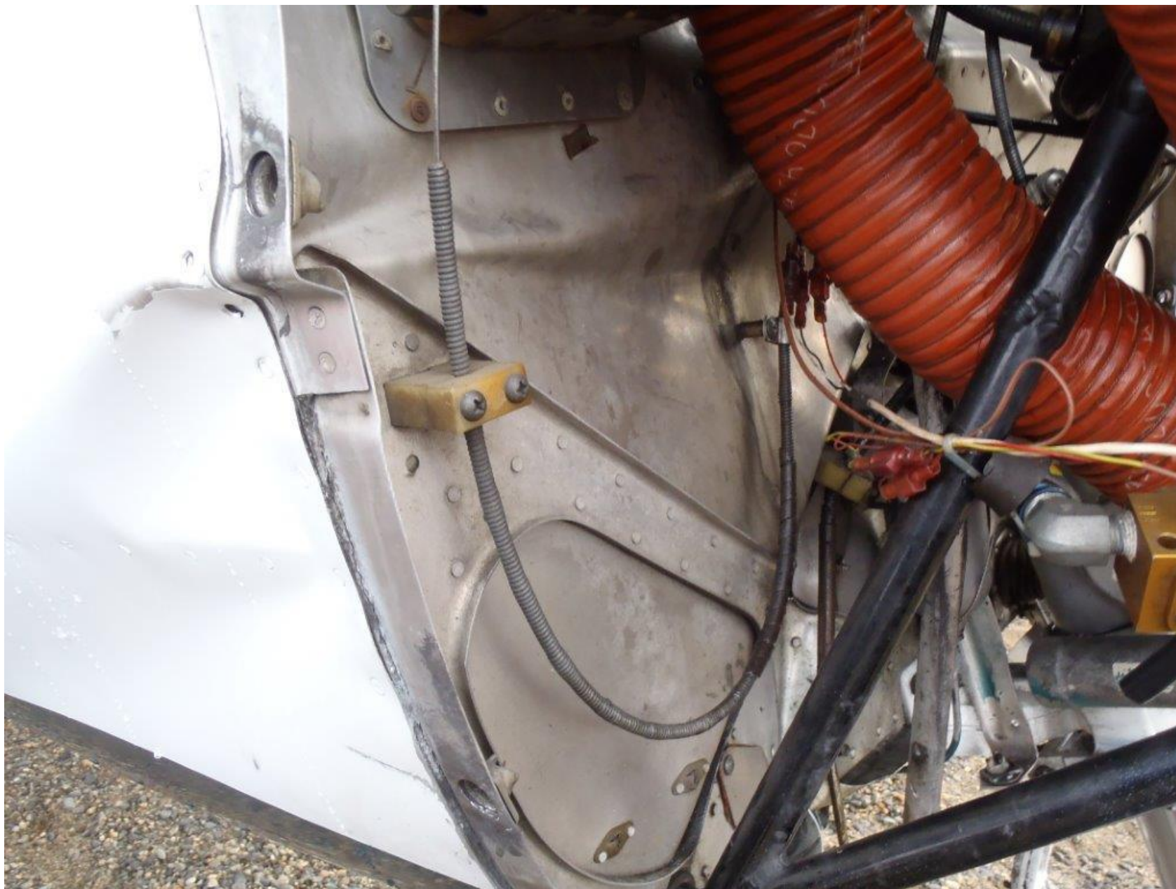
Photo 4 – View of firewall (photo courtesy of the pilot)
