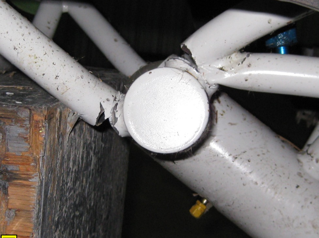
Photo 1 – Engine mounts (Photo Courtesy of FAA)
