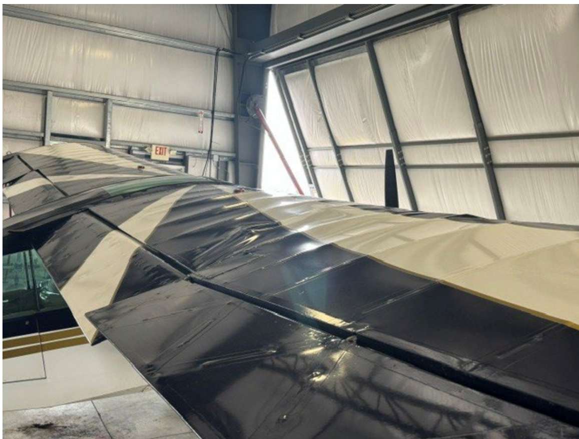
Photograph 2 - Substantial damage to right wing (Courtesy of FAA)
