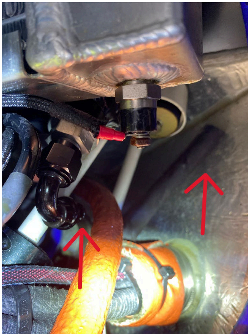
Photograph 4 - Separated Oil Line And Oil Cooler Fitting (Courtesy of FAA)
