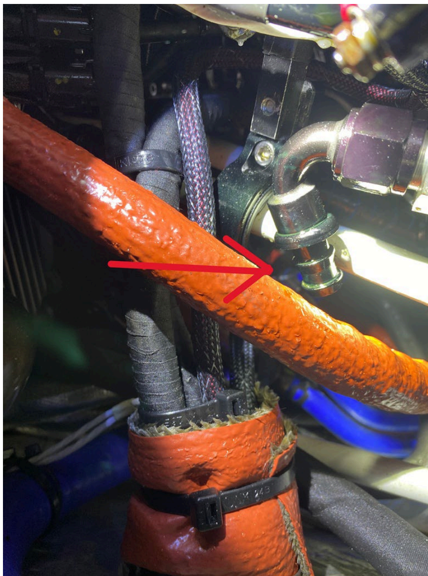
Photograph 5 - Close-up of Oil Cooler Fitting (Courtesy of FAA)
