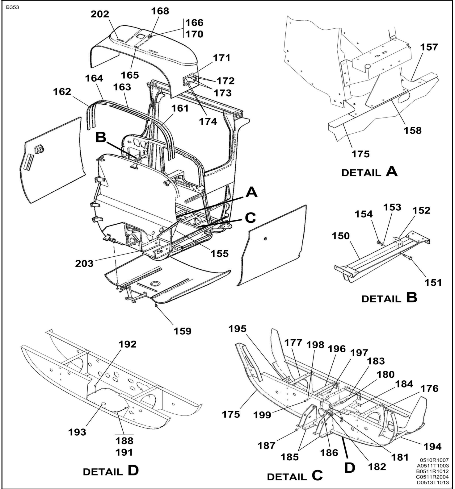
Figure 02 : Sheet 03 : FUSELAGE FRONT SECTION STRUCTURE ASSEMBLY
