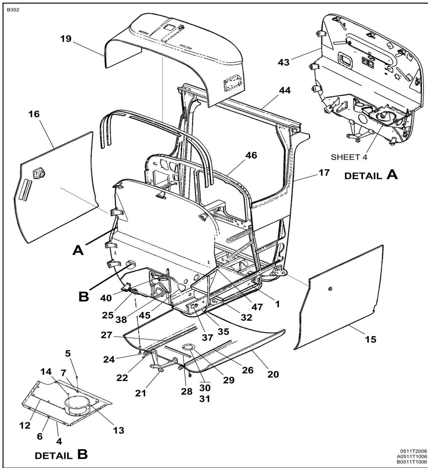
Figure 02 : Sheet 01 : FUSELAGE FRONT SECTION STRUCTURE ASSEMBLY
