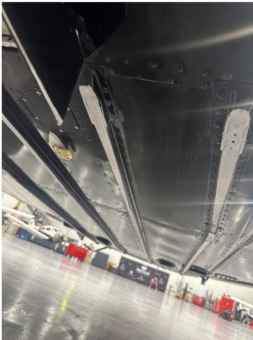
Photograph 2 - Lower External Longeron Damage (Courtesy of FAA)
