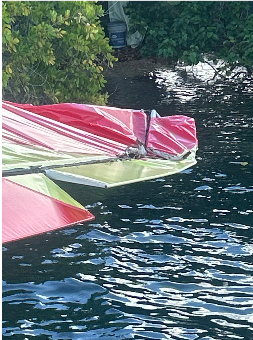
Photograph 2 - Right Wing Damage (Courtesy of FAA)
