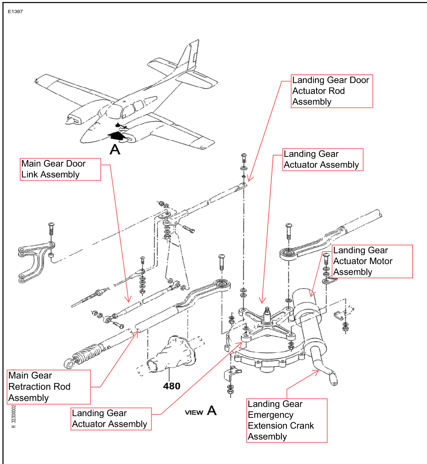
Figure 02 : Sheet 06 : MAIN GEAR RETRACT MECHANISM
