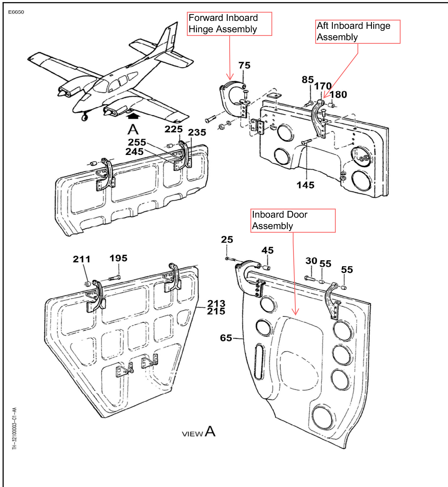
Figure 03 : Sheet 01 : MAIN LANDING GEAR DOORS
