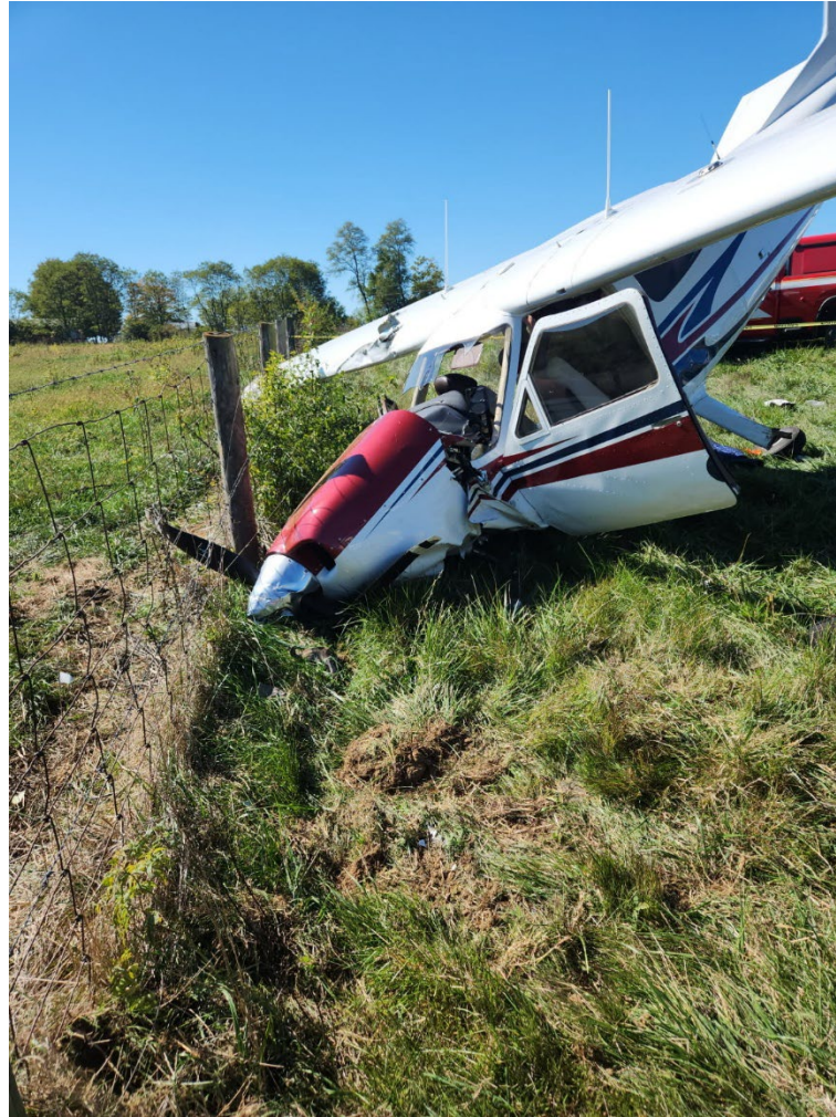
Photograph 2 - View of left side of airplane showing airframe and engine compartment damage. (Courtesy of FAA)
