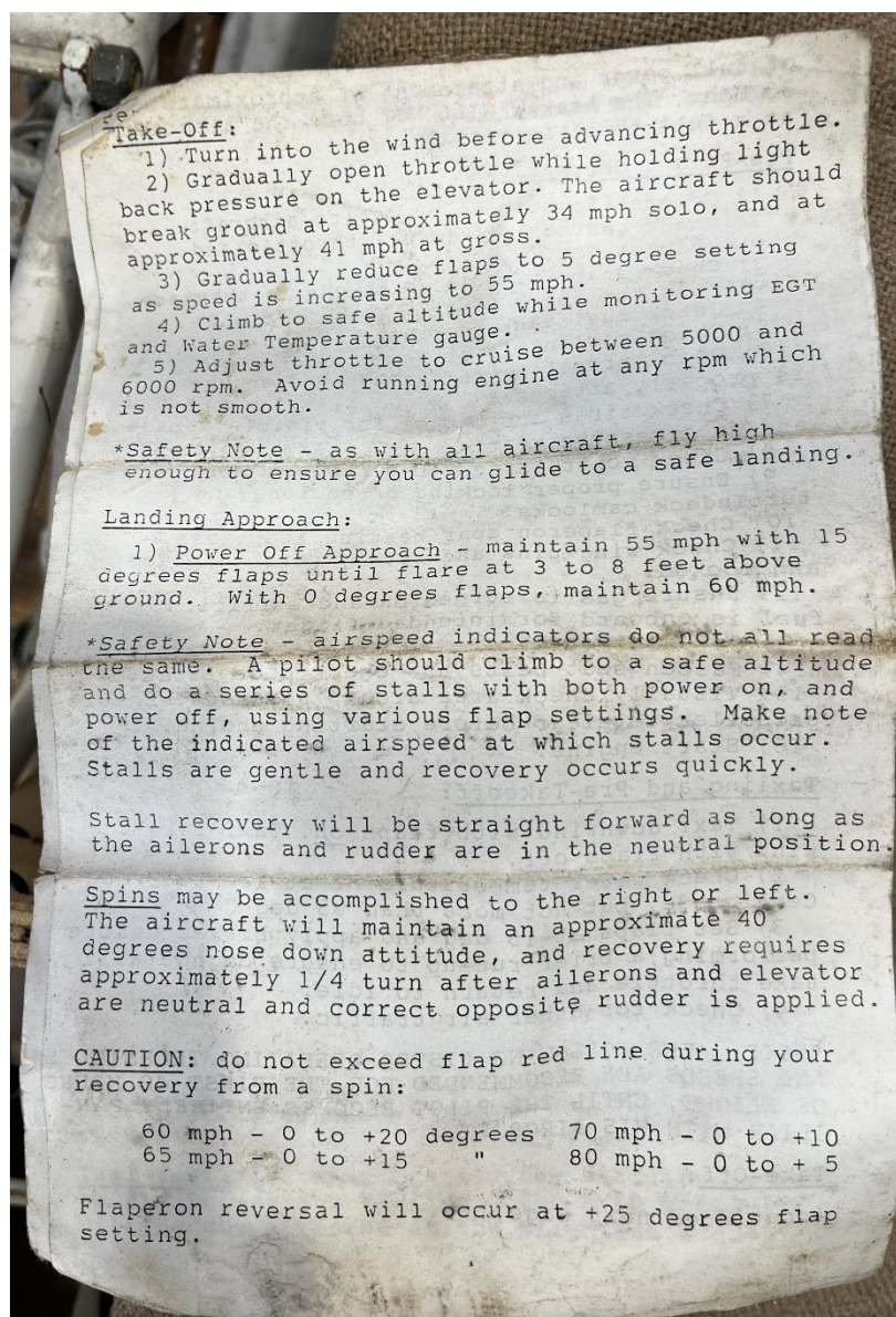
Photograph 4 - Flight Manual Found in N533SE , Specifications, Continued(Courtesy of FAA)
