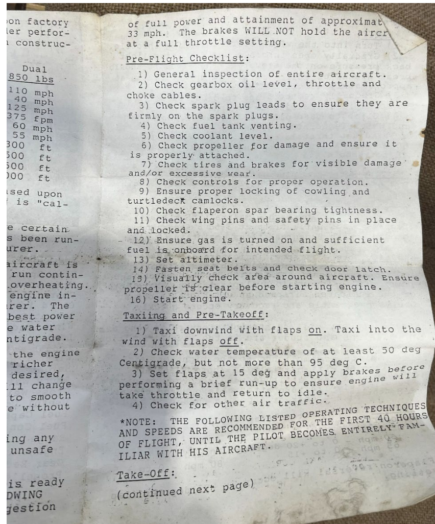
Photograph 3 - Flight Manual Found in N533SE, Procedures (Courtesy of FAA)
