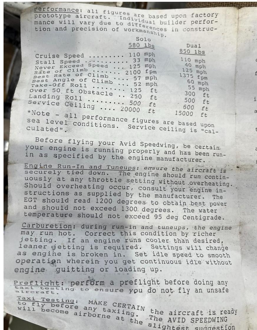
Photograph 2 - Flight Manual Found in N533SE, Performance Information (Courtesy of FAA)
