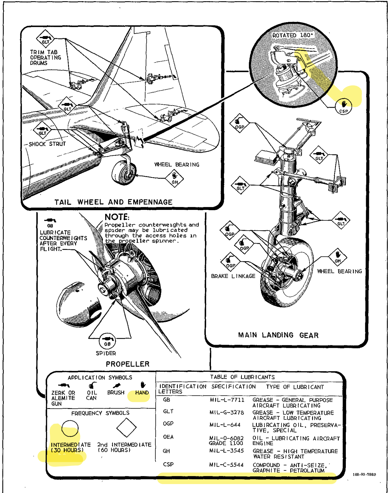
Figure 3-10 (Sheet 1 of 3 Sheets). Lubrication Chart
