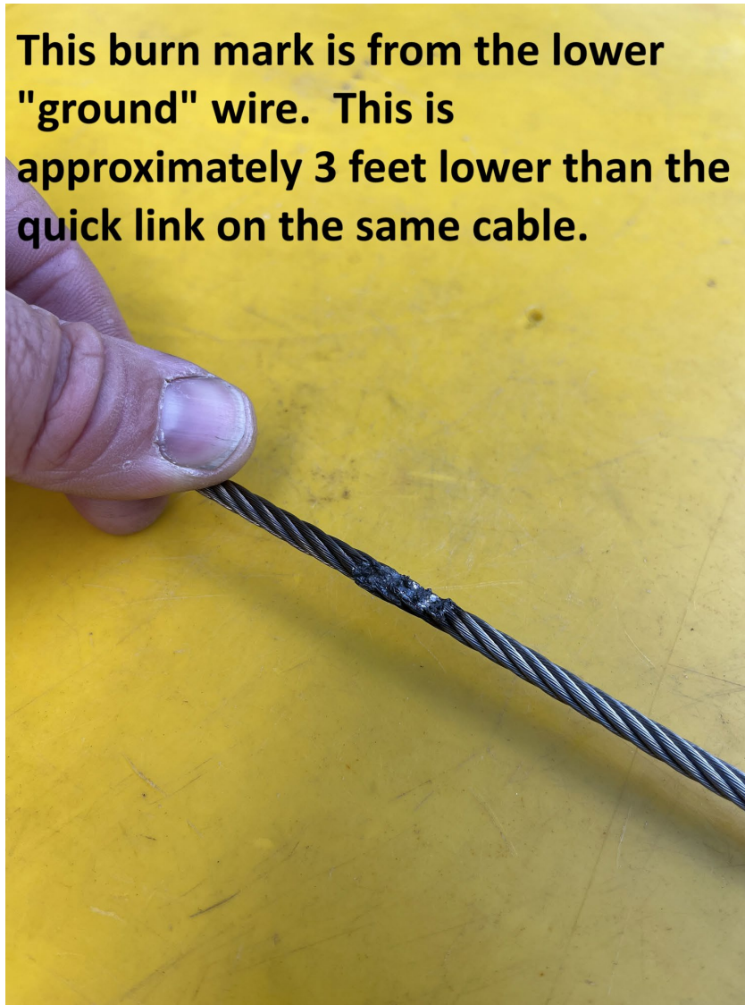
Photograph 2 - Burnt cable (Courtesy of Owner)
