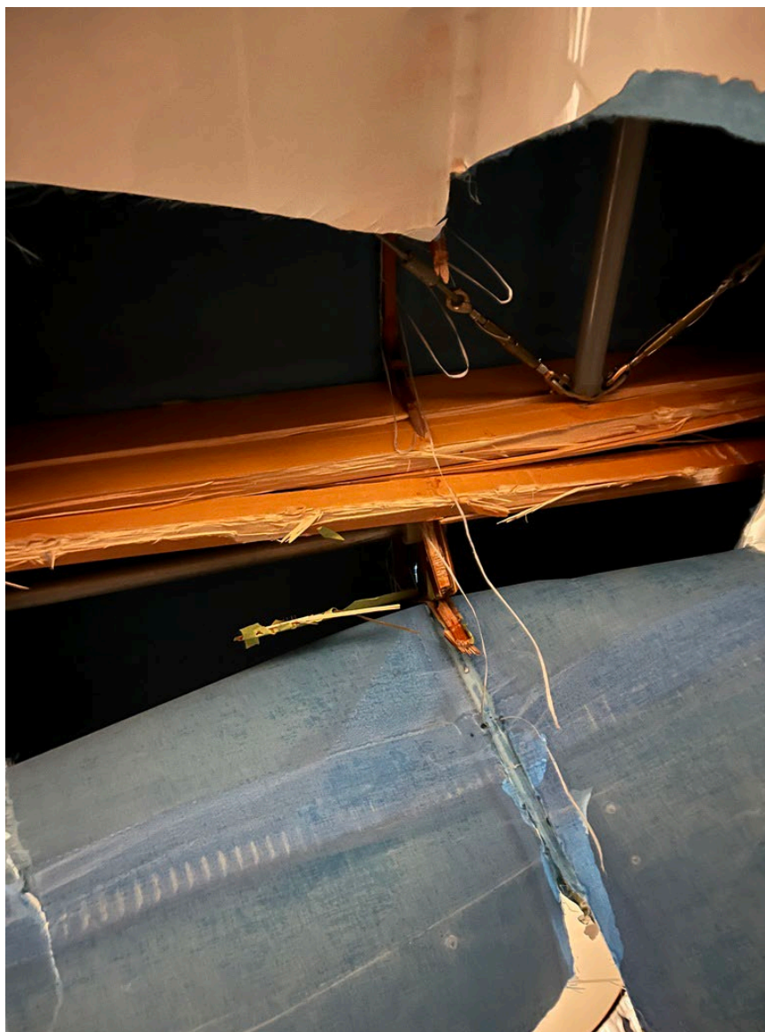
Photograph 2 - Left Wing Spar Damage (Courtesy of FAA)
